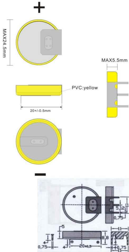
Fig1. Structure of CR2450
