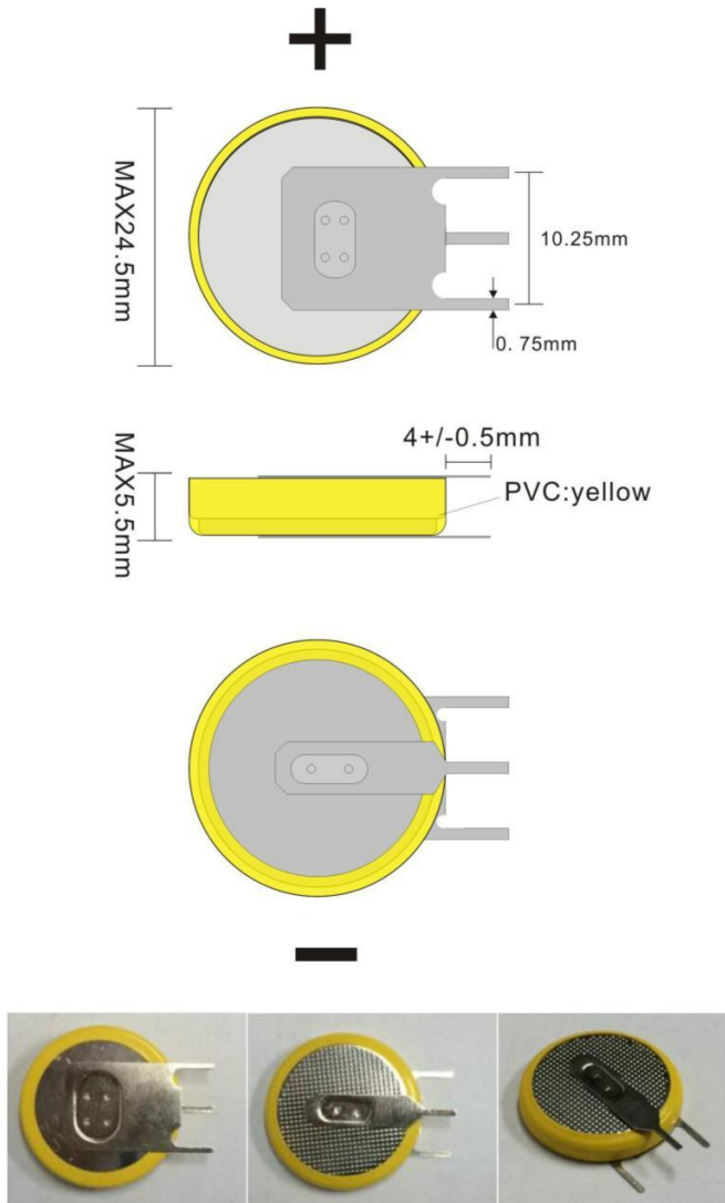
Fig1. Structure of CR2450
